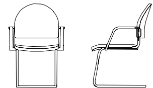
AR2B | Stackable Cantilever with Arms.
